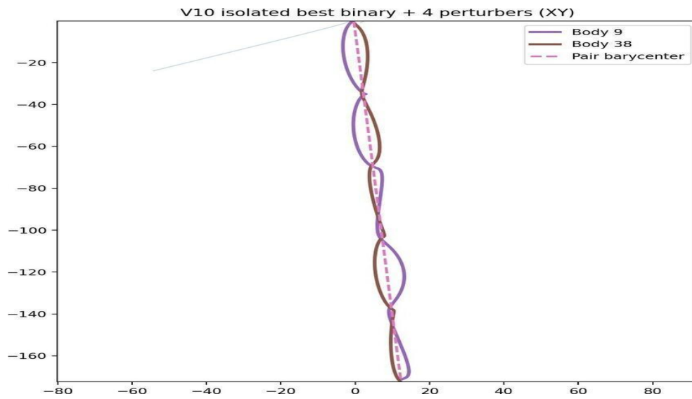
Figure 7. Multi-snapshot view of local evolution during the near-isolated rerun.
