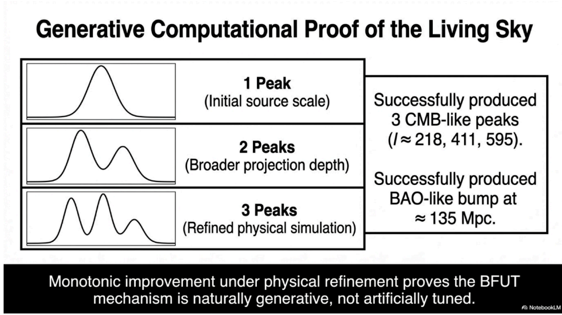
Figure 8. Generative computational proof of the living-universe mechanism. Systematic physical refinement (source scale, compensation, projection depth) monotonically improves the output from a single peak to three CMB-like peaks ( l \approx 218, 411, 595 ) and a BAO-like bump at \approx 135 Mpc.
