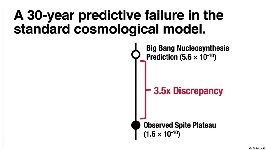
Figure 3. Conceptual comparison between the Standard Model (BBN) and the BFUT steady-state framework.
