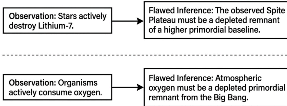
Figure 6. The cosmological lithium problem is resolved under the BFUT steady-state framework without new physics.
