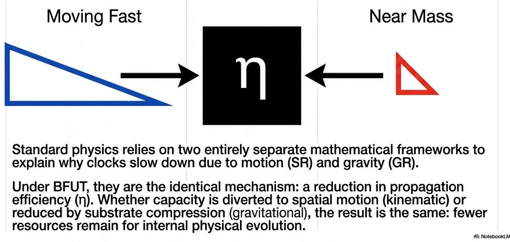
Figure 6: The Grand Unification: Both kinematic and gravitational time dilation arise from the same mechanism - reduction in propagation efficiency \eta .
