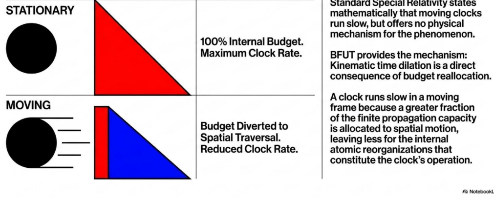
Figure 4: Special Relativity demystified: Moving clocks run slow because a greater fraction of the finite propagation budget is allocated to spatial motion.
