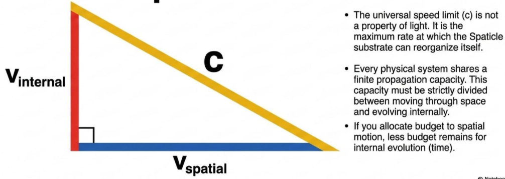
Figure 2: The Propagation Budget: c^2 = v_{\text{spatial}}^2 + v_{\text{internal}}^2 . Capacity allocated to spatial motion reduces the budget available for internal evolution (time).
