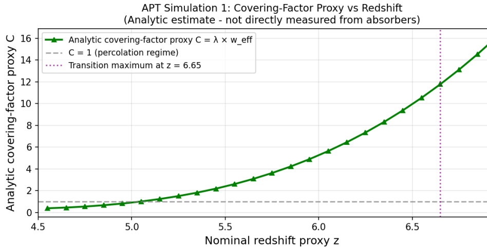
Figure 1c. APT Simulation 1 - Analytic covering-factor proxy C = \lambda \times w_{\text{eff}} vs redshift. C rises well above unity before the transition, consistent with the percolation threshold mechanism. Note: C is an analytic estimate from parametric formulas, not directly measured from the simulated absorbers.
