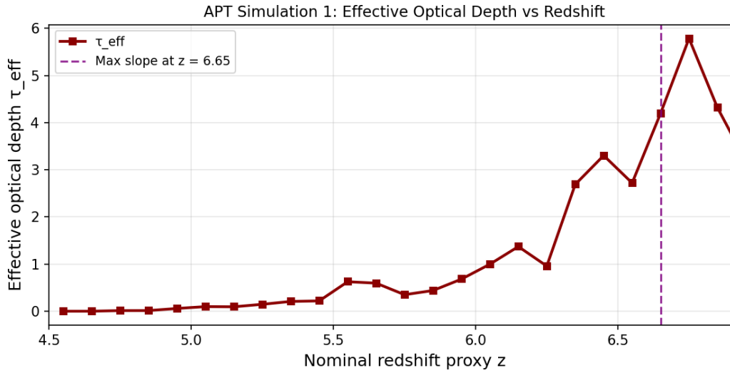
Figure 1b. APT Simulation 1 - Effective optical depth vs redshift. Maximum steepening occurs at z \sim 6.65 with a slope of 15.3 per unit redshift, demonstrating the sharply nonlinear nature of the APT transition from a smooth absorber gradient.
