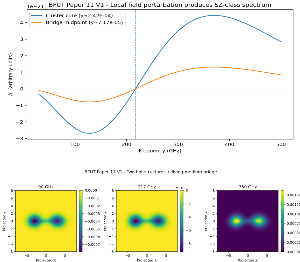
Simulation 1: BFUT forward model reproducing the SZ-class signal (low-frequency decrement, crossover near 218 GHz, high-frequency increment, and bridge-like excess) from local Sparticle field interaction with hot plasma nodes.
